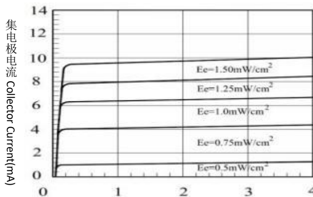
Collector Current vs. Collector-Emitter Voltage
