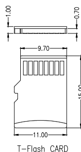
T-Flash CARD
