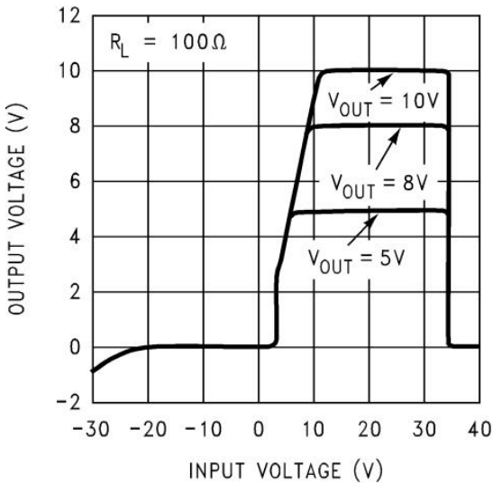
Figure 15. Output at Voltage Extremes
