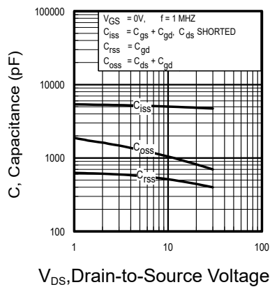
Figure 5: Typical Output Characteristics
