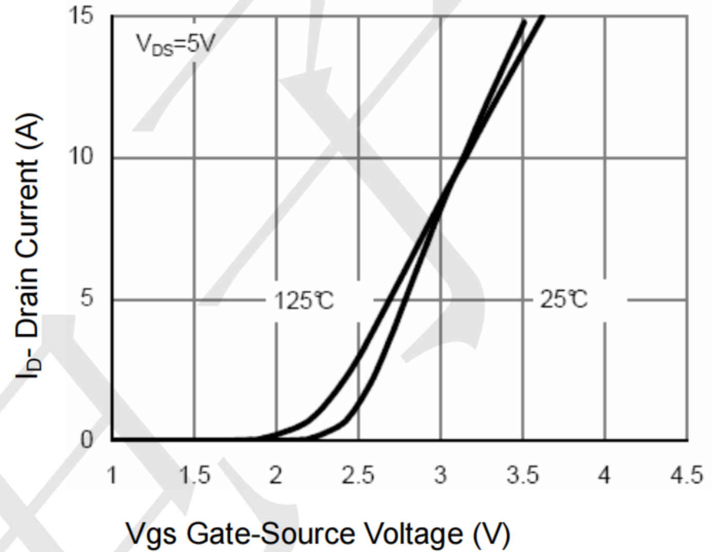
Figure 2 Transfer Characteristics
