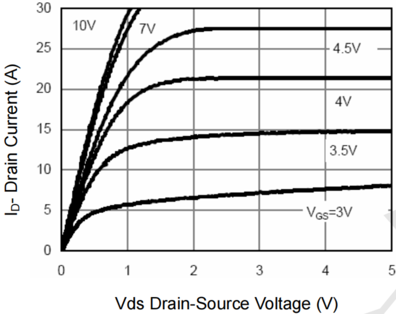
Figure 1 Output Characteristics
