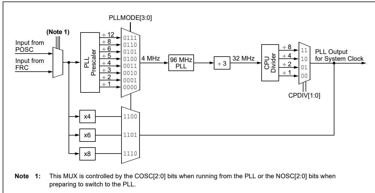
FIGURE 9-2: PLL BLOCK
