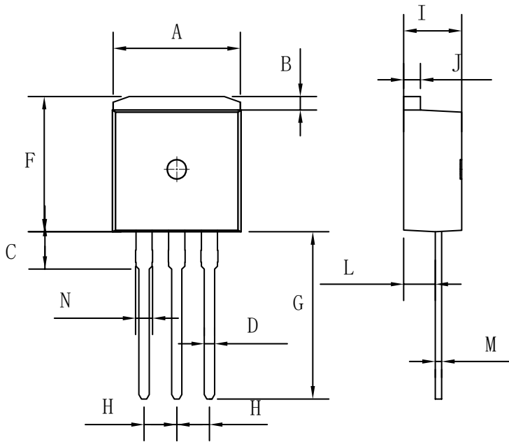
TO-262
