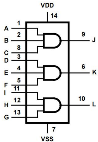
Figure 2.2 Functional Diagram
