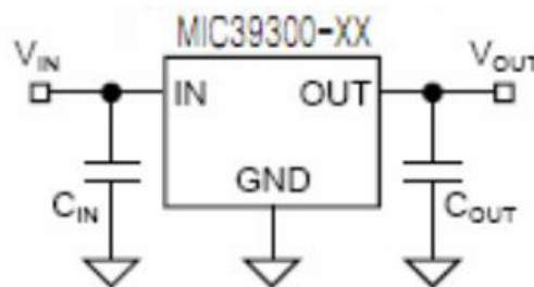
Fig 1. Capacitor Requirements
