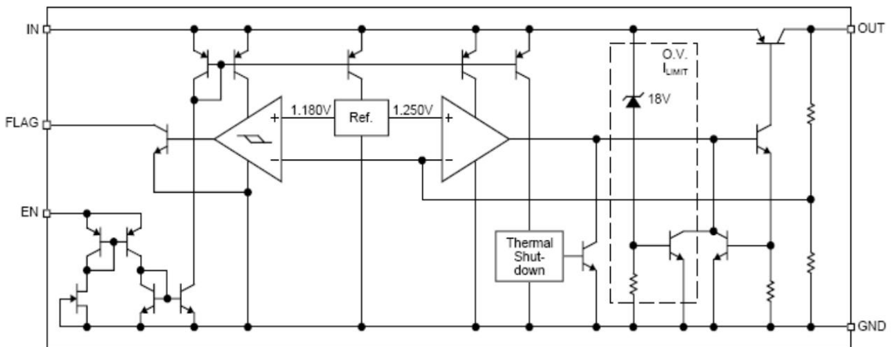
MIC39301 Fixed with flag and enable
