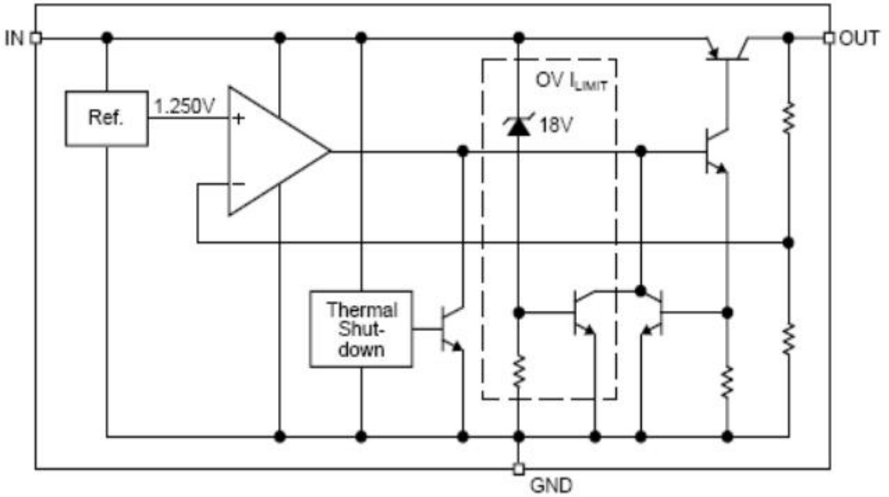
MIC39300 Fixed (1.5V,1.8V,2.5V,3.3V,5.0V)
