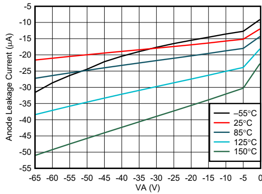
Figure 7-7. ANODE Leakage Current vs Reverse ANODE Voltage
