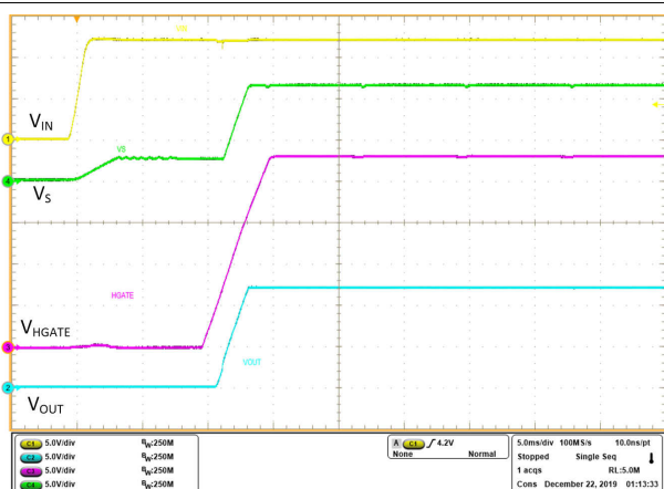
Figure 10-25. Power up 12 V - HGATE and Output
