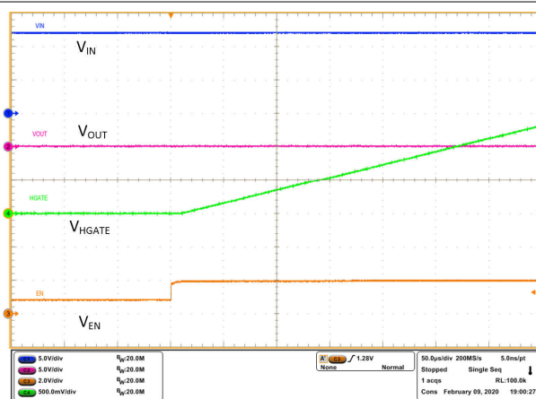
Figure 10-15. Turn ON delay - HGATE
