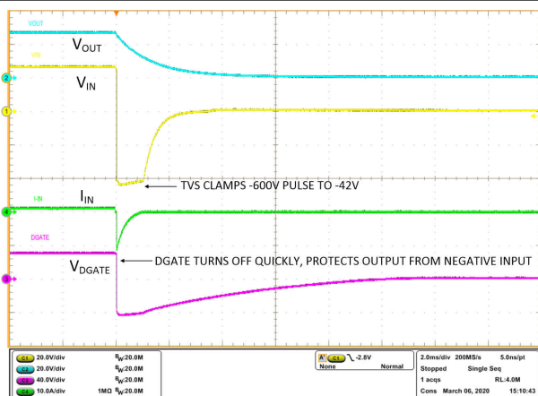
Figure 10-23. ISO 7637-2 Pulse 1 –600 V 50 Ω
