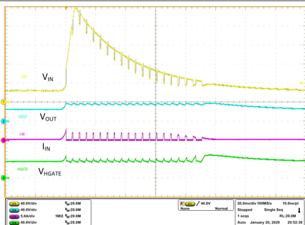
Figure 10-21. Unsuppressed Load Dump 200 V - Output Clamp
