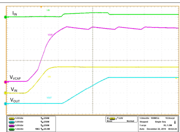
Figure 10-3. Startup 12 V showing Charge Pump VCAP
