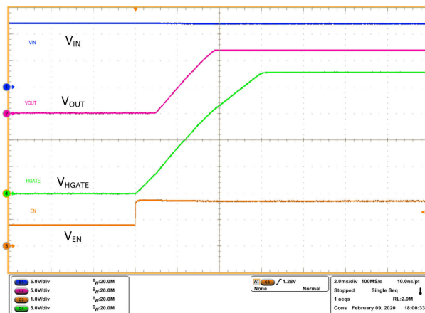
Figure 10-11. Turn ON with VCAP ON - EN rising from 0.8 V
