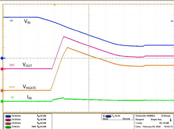
Figure 10-14. Overvoltage Recovery
