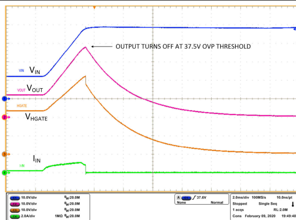
Figure 10-13. Overvoltage Protection
