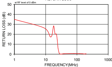
SCLF-21.4 RETURN LOSS
