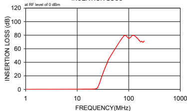
SCLF-21.4 INSERTION LOSS
