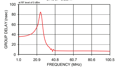
SCLF-21.4 GROUP DELAY
