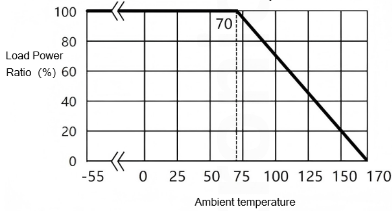
Power curve
