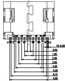
USB TYPE-C PIN ASSIGNMENTS
