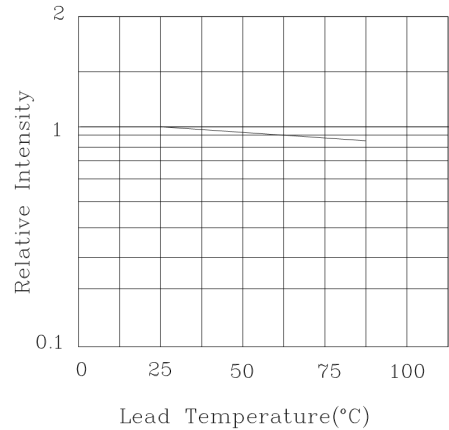
RELATIVE INTENSITY VS. LEAD TEMPERATURE
