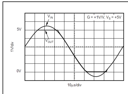
FIGURE 3. HXA348A—No Phase Inversion with Inputs Greater than the Power-Supply Voltage.
