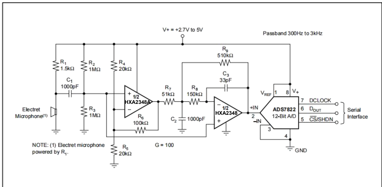
FIGURE 8. HXA2348A as a Speech Bandpass Filtered Data Acquisition System.
