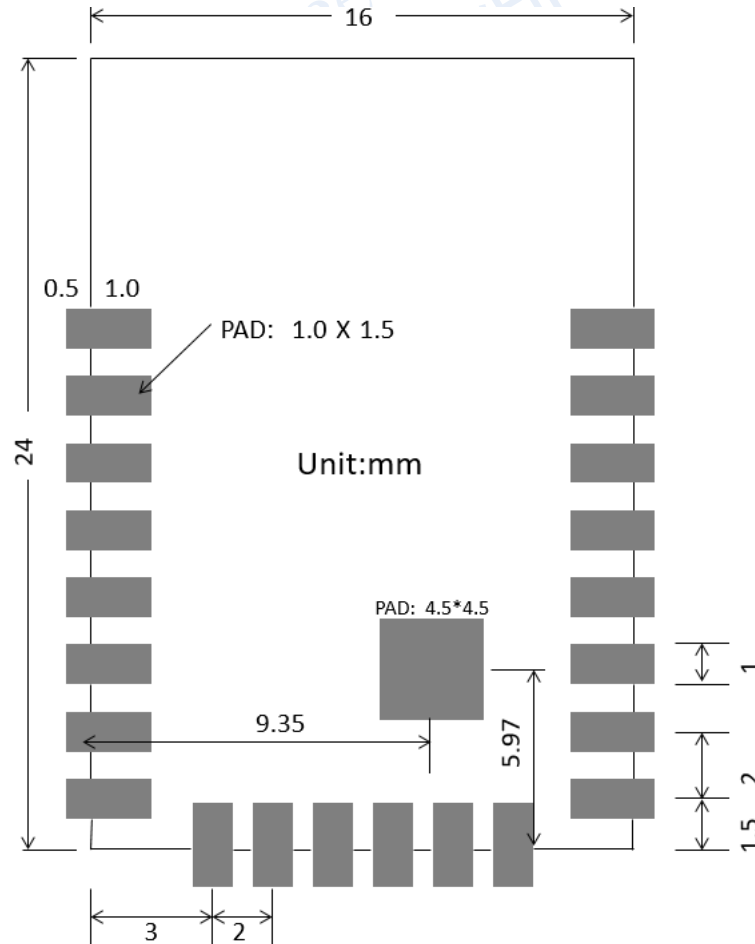
Fig. 3.3 PCB Layout for ESPC5-12E (Top view)
