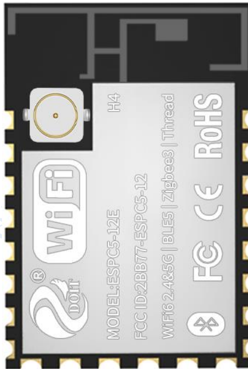
Fig.3.1 Shape for ESPC5-12E
