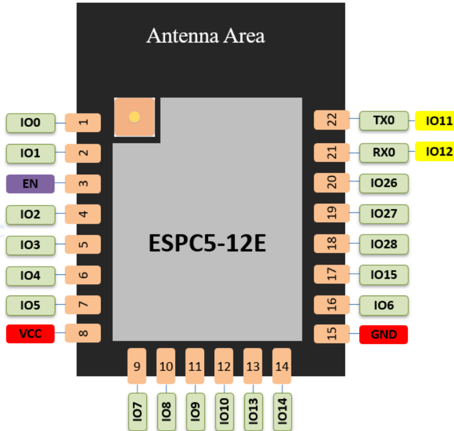
Fig.2.1 ESPC5-12E Pins Definition (Top view)
