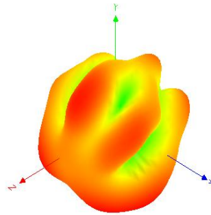
Frequency (MHz) : 1570
