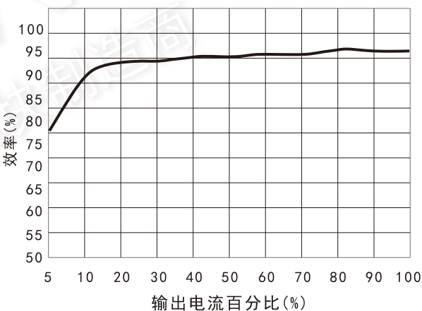
效率Vs输出负载(Vin=48V) VRB4815LD-15WR3
