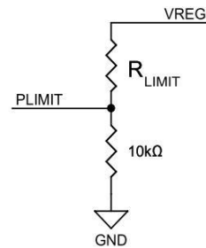
Figure 2. PLIMIT Pin Voltage Divider Use the simple voltage divider to determine the voltage on PLIMIT pin from VREG pin by the following equation:
