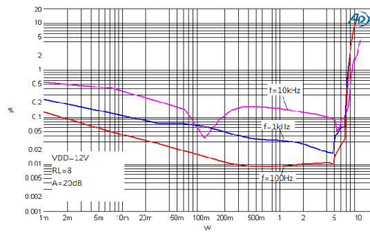
Figure 15. THD+N vs. Output Power
