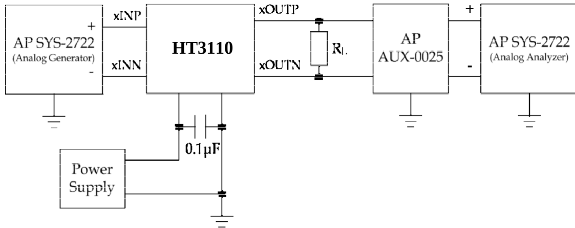
Test Setup Connection Diagram
