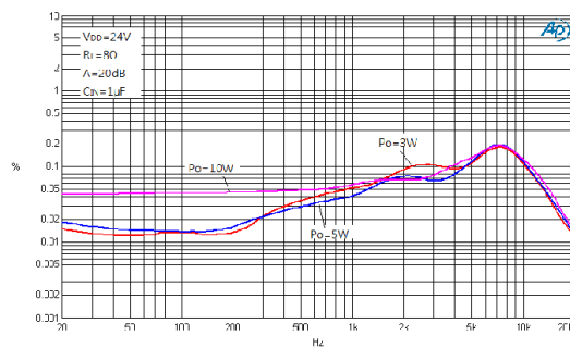
Figure 10. THD+N vs. Frequency
