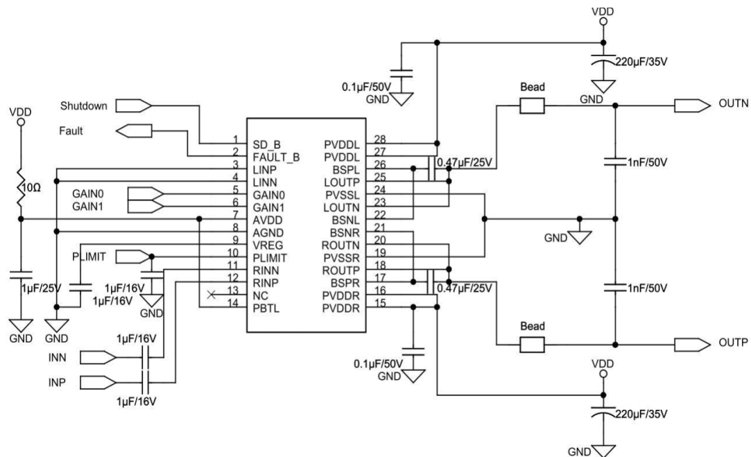
Figure 26. HT3110 Mono Reference Application Circuit
