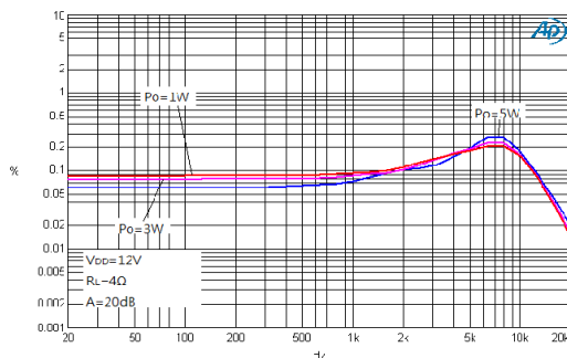
Figure 19. THD+N vs. Frequency
