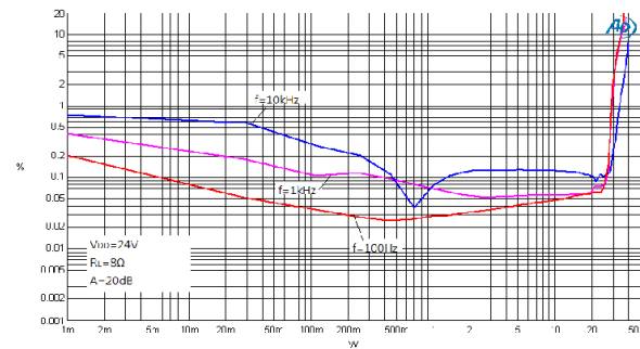
Figure 16. THD+N vs. Output Power
