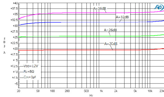
Figure 7. Frequency Response
