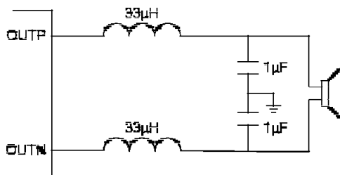
Figure 3. Typical LC Output Filter, Speaker Impedance= 8\Omega
