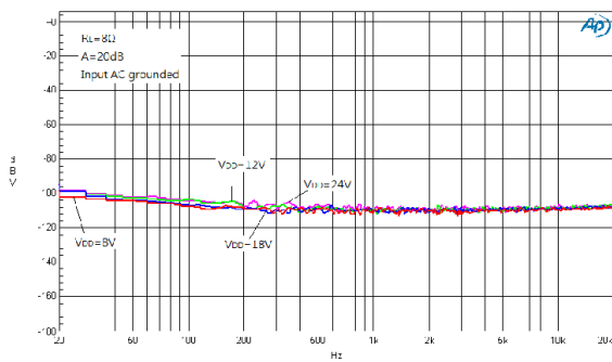
Figure 11. Crosstalk
