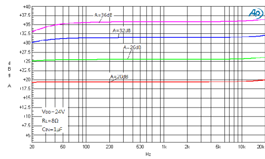
Figure 8. Frequency Response
