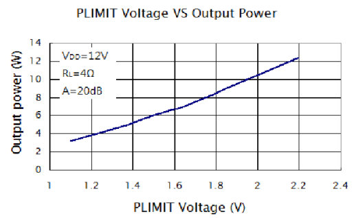
Figure 24. PLIMIT voltage vs. Output Power
