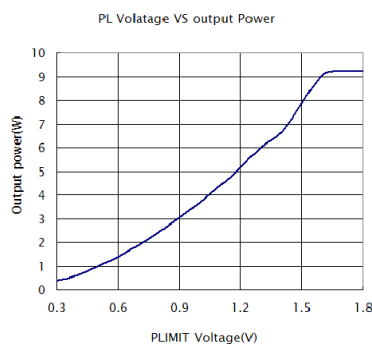
Figure 17. PLIMIT voltage vs. Output Power
