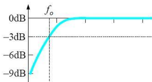
Figure 1. Cut-off Point of High-pass Filter
