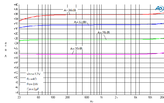
Figure 18. Frequency Response
