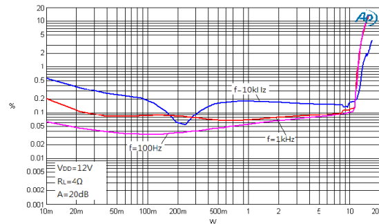
Figure 20. THD+N vs. Output Power
