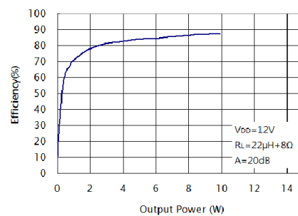
Efficiency VS Output Power
