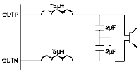
Figure 4. Typical LC Output Filter, Speaker Impedance= 4\Omega
