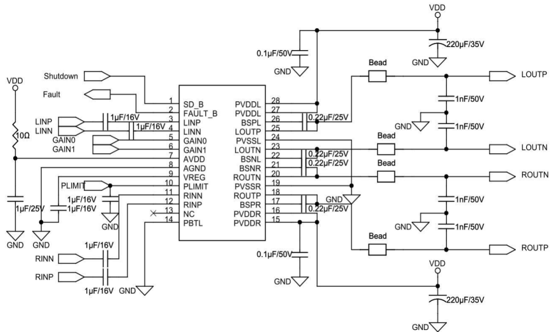
Figure 25. HT3110 Stereo Reference Application Circuit
