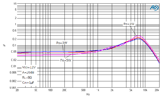
Figure 9. THD+N vs. Frequency
