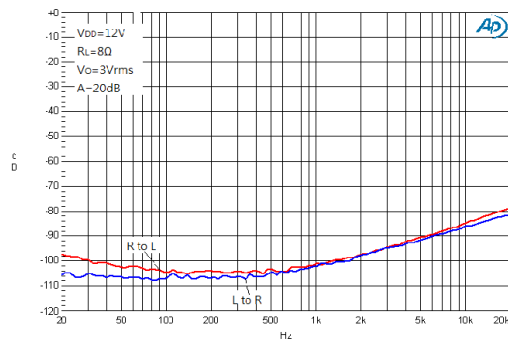
Figure 11. Crosstalk
