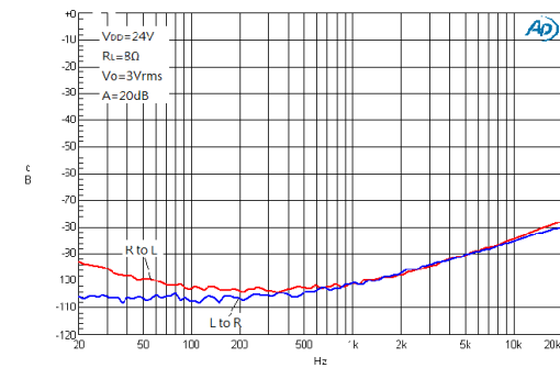
Figure 12. Crosstalk
