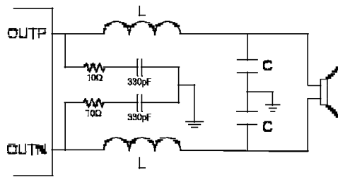
Figure 6. Output Snubber Circuits
