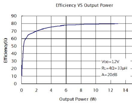
Figure 23. Efficiency
