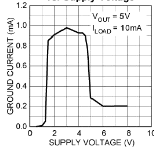
2915x Ground Current vs. Supply Voltage
