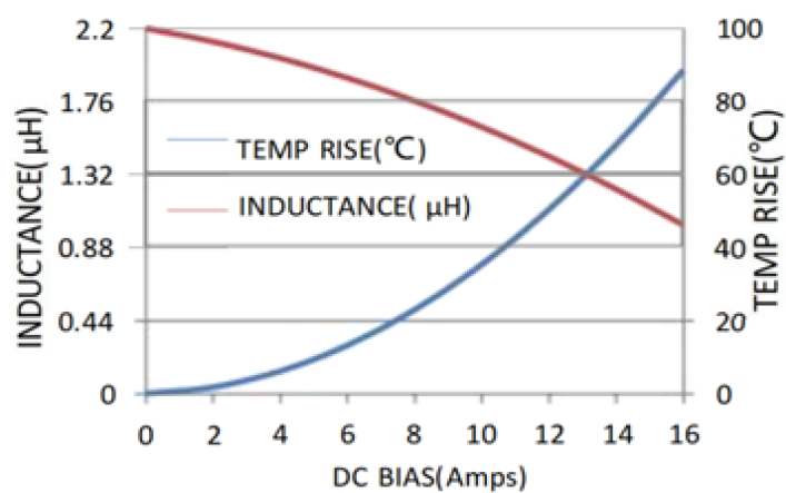
HNRA-4012S-2R2-MT
