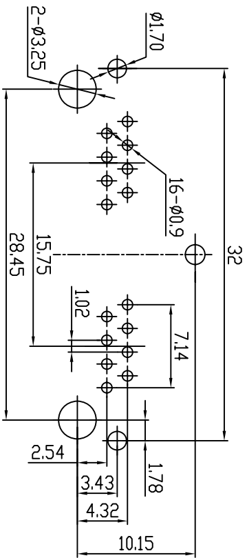
PC Board Layout
