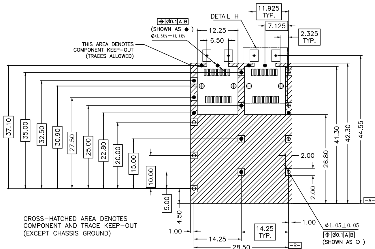
PCB LAYOUT FOR SINGLE SIDE MOUNTING
