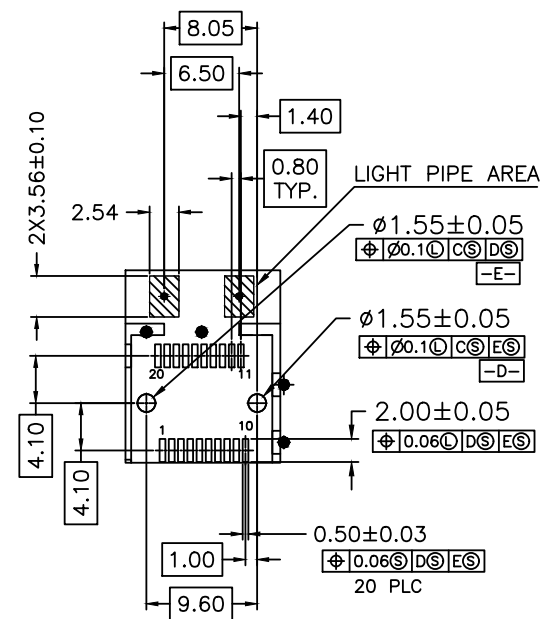
DETAIL H RECOMMENDED CONNECTOR LAYOUT 4X INDIVIDUALLY
