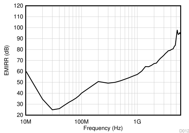
Figure 6-1. EMIRR Testing
