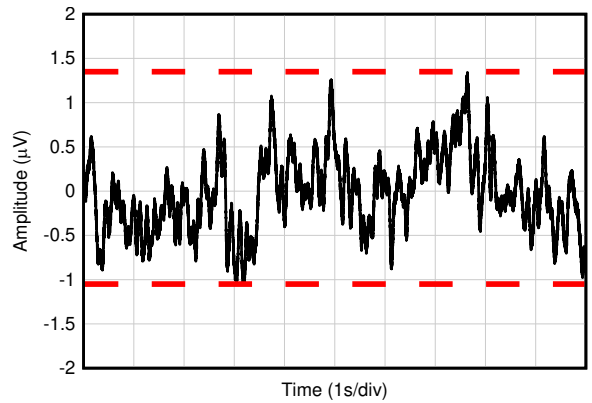
Figure 5-20. 0.1Hz to 10-Hz Noise
