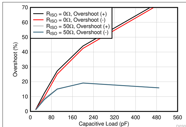
Figure 6-3. Small-Signal Overshoot vs Capacitive Load (20mV pp Output Step, G = +1)
