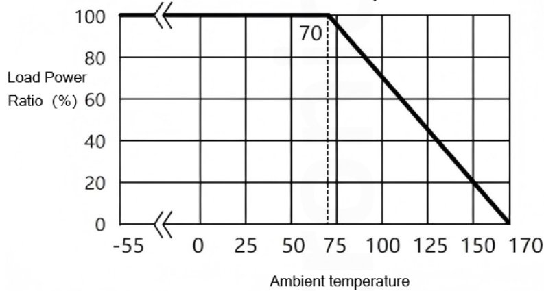
Power curve
