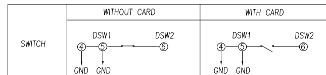
CRICUIT DIAGRAM FOR CARD DETECT SWITCH
