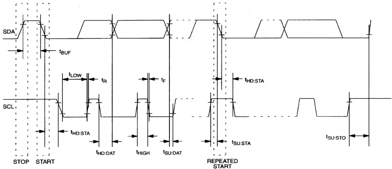
Figure 2: Timing Diagram
