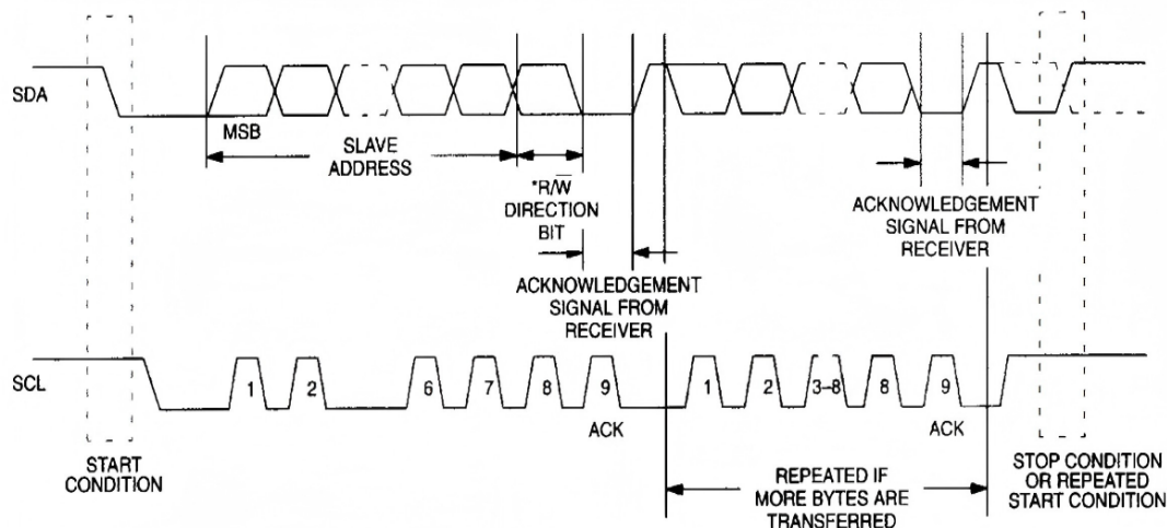
Figure 6 : Data Transfer on I 2 C Serial Bus
