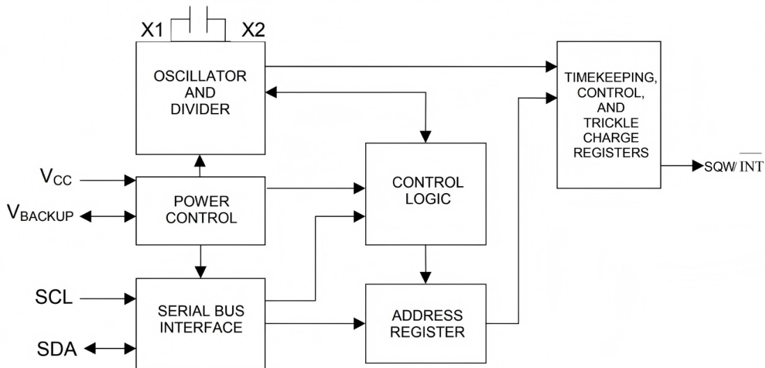
Figure 4: Block Diagram
