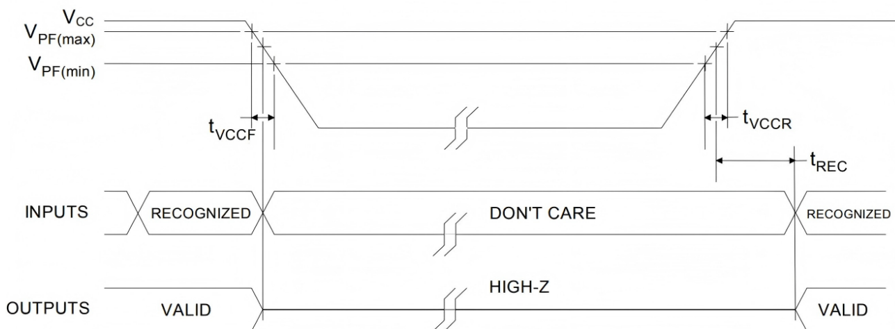
Figure 3: Power-Up/Power-Down Timing
