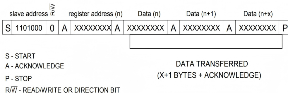
Figure 7 : Data Write—Slave Receiver Mode
