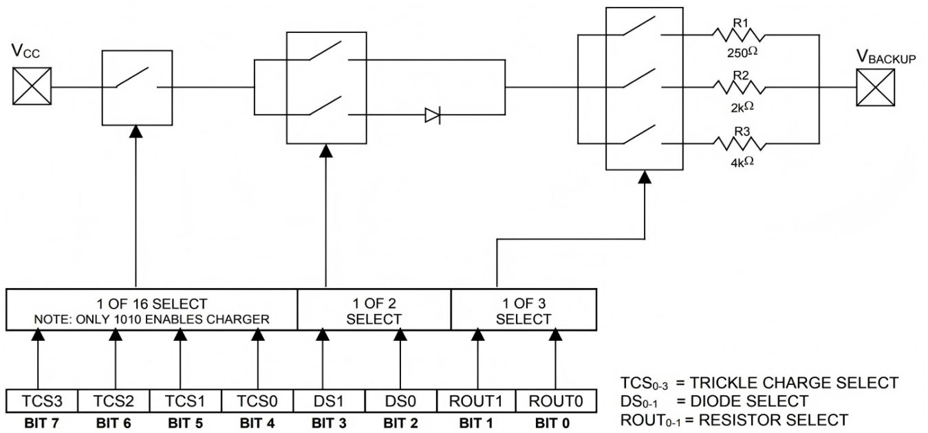
Figure 5: Programmable Trickle Charge
