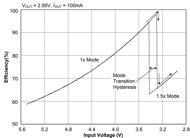
Efficiency — 100mA
