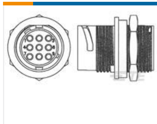
TE Part #1445816-1 RECP,11-9,FLNG MT,STD KEY
