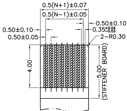
APPLICABLE FPC/FFC RECOMMENDED DIMENSION (THICKNESS:0.30±0.03)
