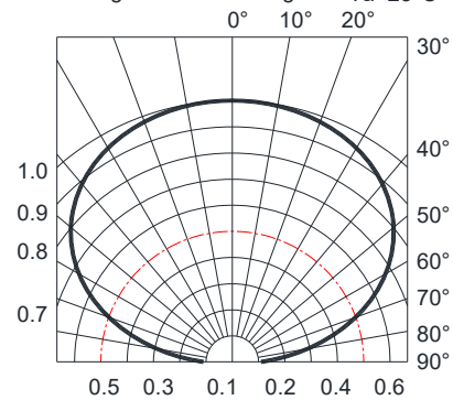
Fig.6-Radiation Diagram T_a=25^{\circ}\text{C}
