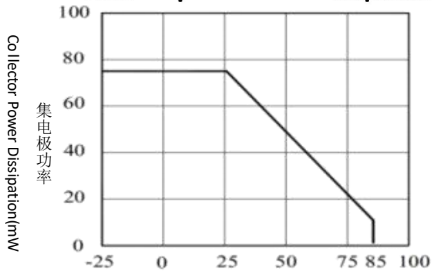
Collector Power Dissipation vs. Ambient Temperature
