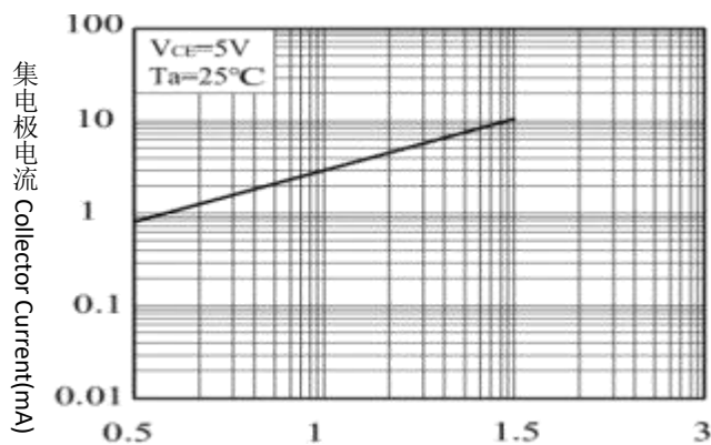
Collector Current vs. Irradiance
