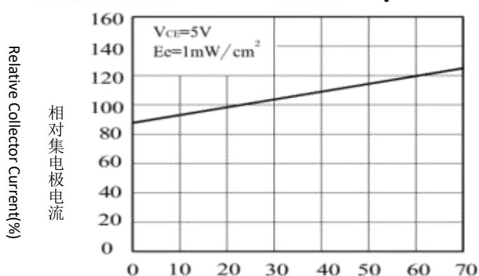
Relative Collector Current vs. Ambient Temperature
