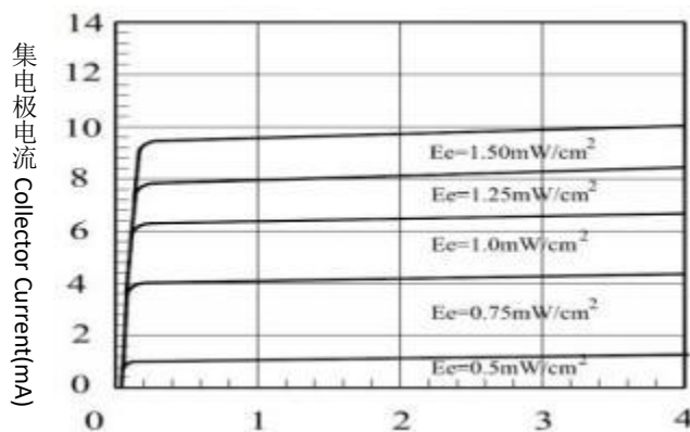
Collector Current vs. Collector-Emitter Voltage
