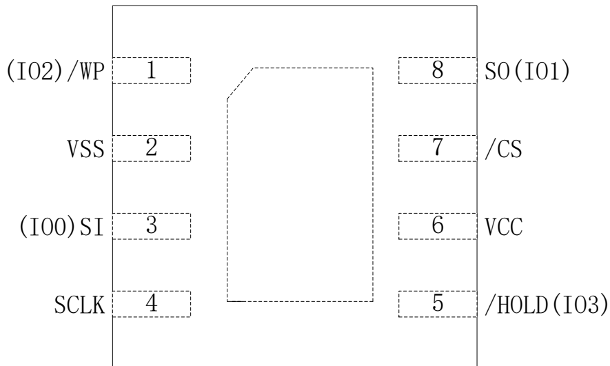
Figure 3.b. Pin Configuration DFN 1.5*1.5mm
