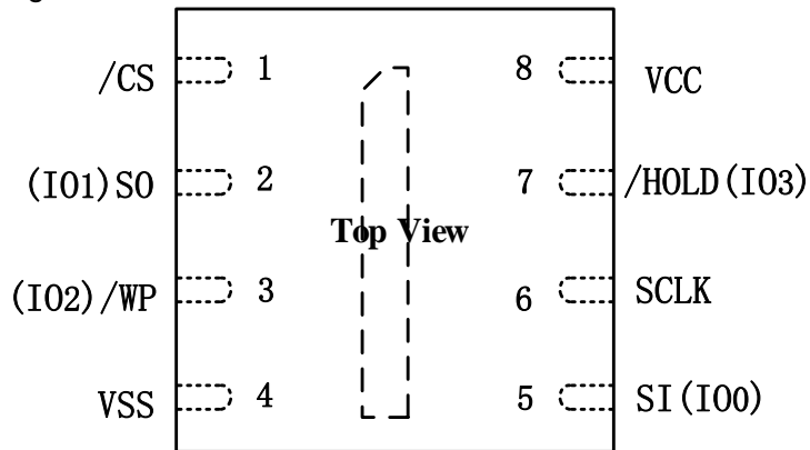
Figure 3.a. Pin Configuration DFN 2*3mm
