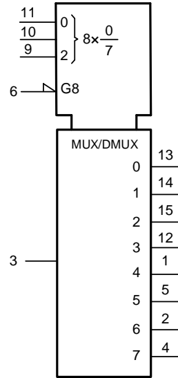
Figure 8-2 IEC logic symbol
