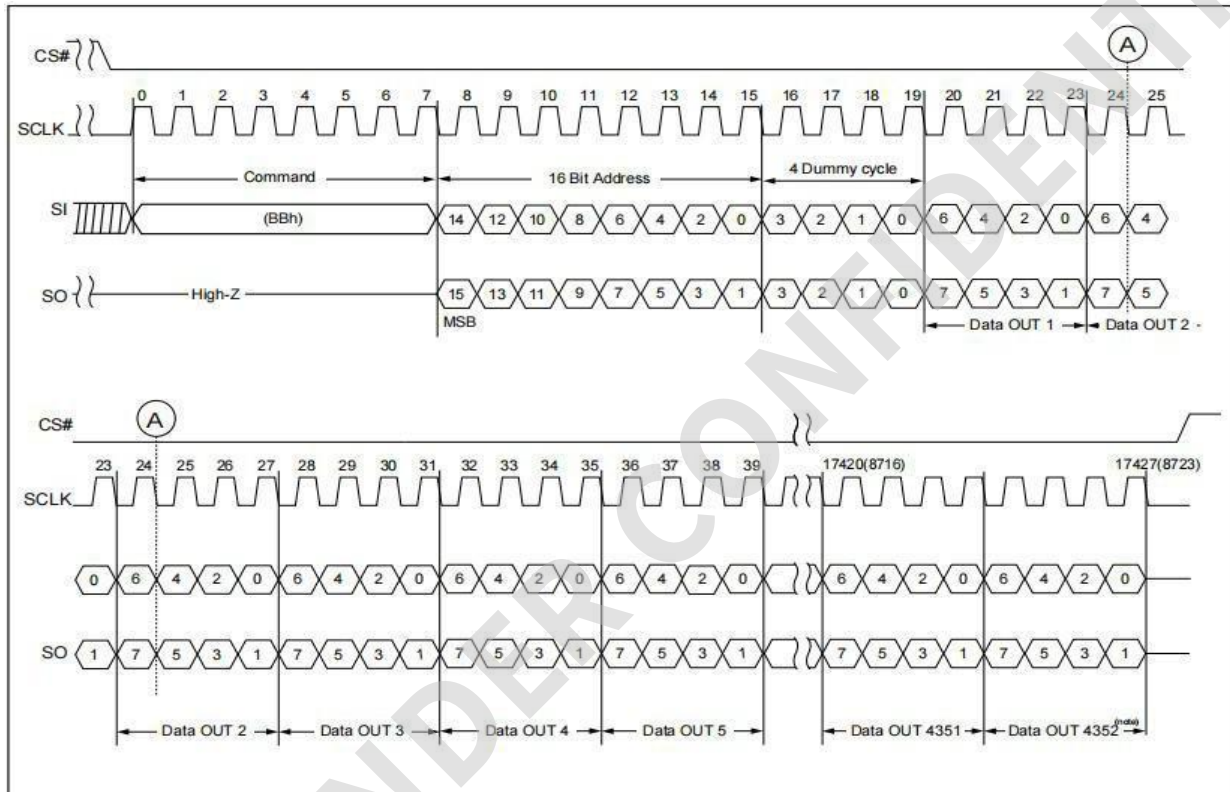
Figure 8-9. Read From Cache Dual IO Timing Diagram
