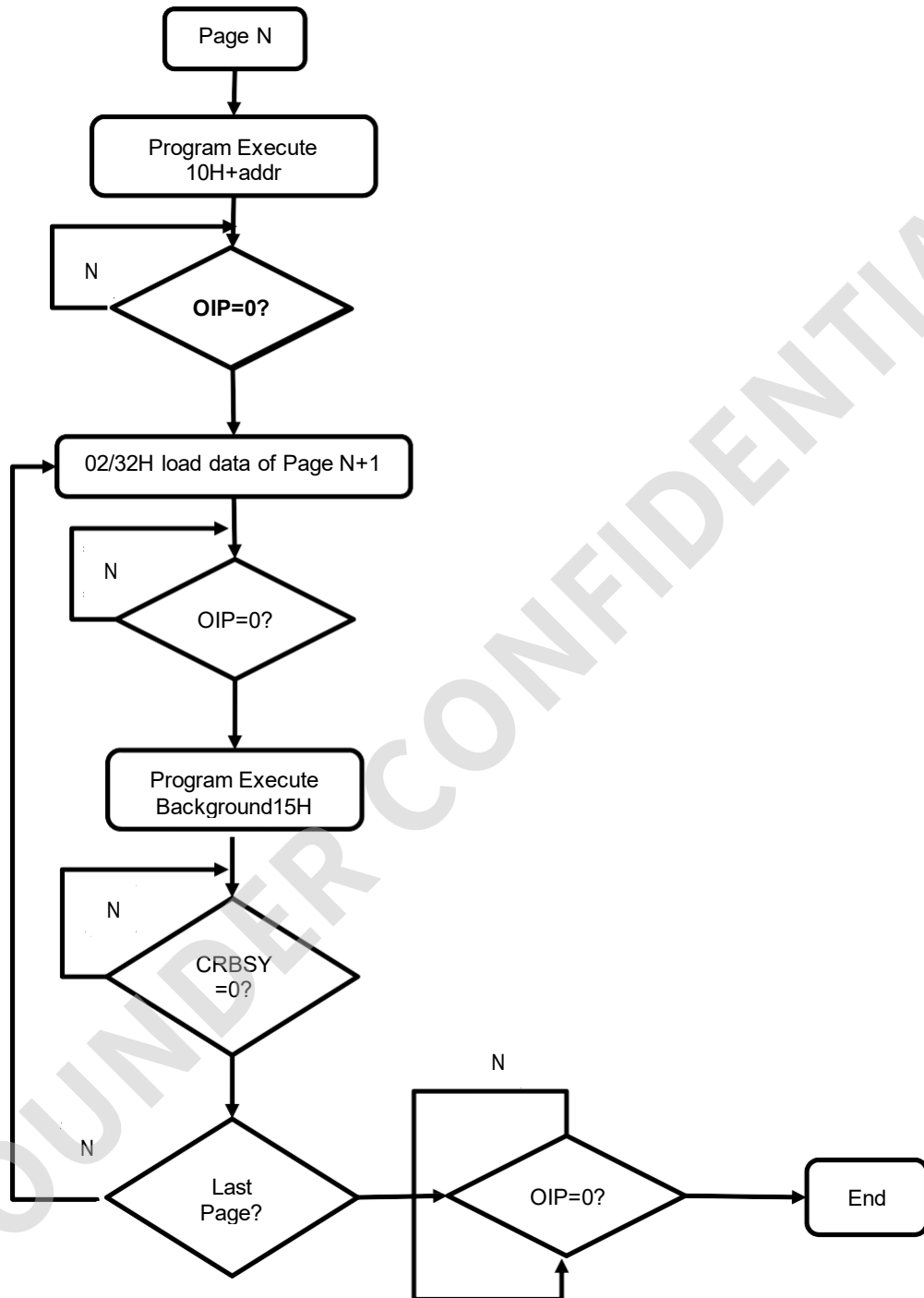
Figure 9-4. Program Execute Background Sequential Timing Diagram
