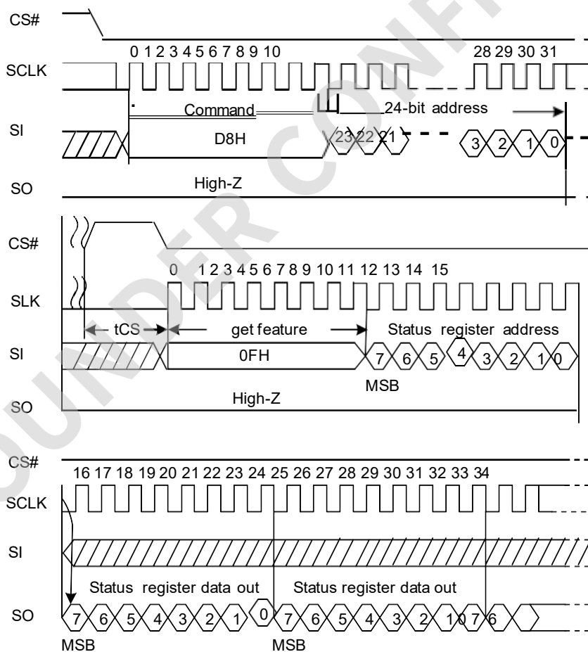
Figure 10-1. Block Erase Timing Diagram
