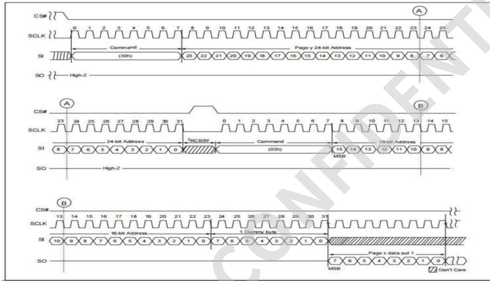
Figure 8-3. Read Page Cache Sequential Timing
