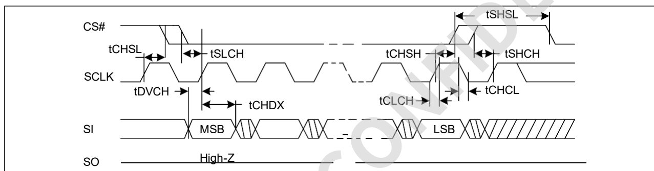
Figure 20-1.Serial Input Timing
