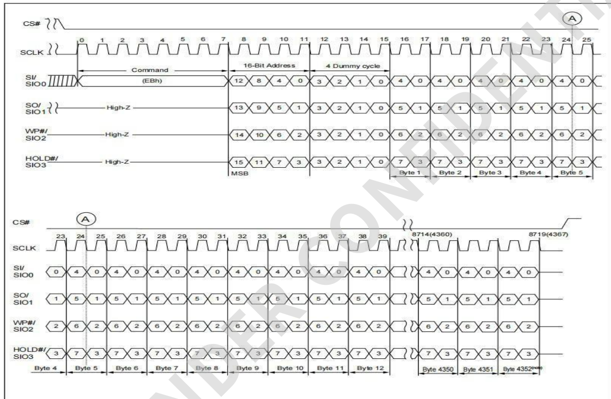
Figure 8-10. Read From Cache Quad IO Timing Diagram
