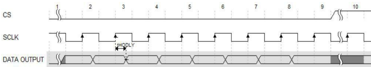
Figure 20-3. Output Timing(HSOD=1)
