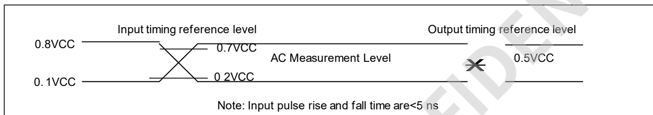
Figure 17-1. Input Test Waveform and Measurement Level
