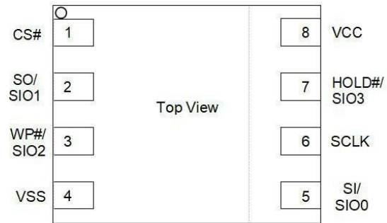
Figure 2-1.Connect Diagram
