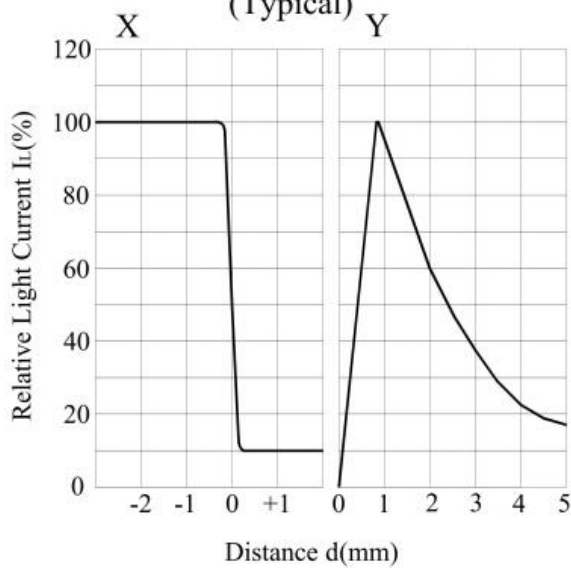
Fig.7 Sensing Position Characteristics (Typical)
