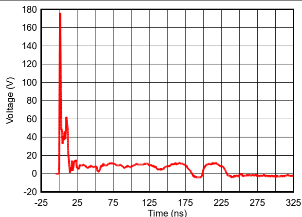
Figure 5-12. +8kV Clamped IEC Waveform (DPY)
