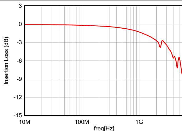
Figure 5-8. Insertion Loss (DPL)
