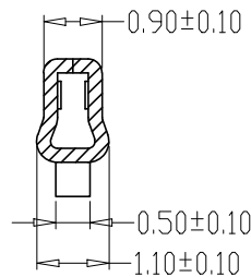
SEC:C-C
