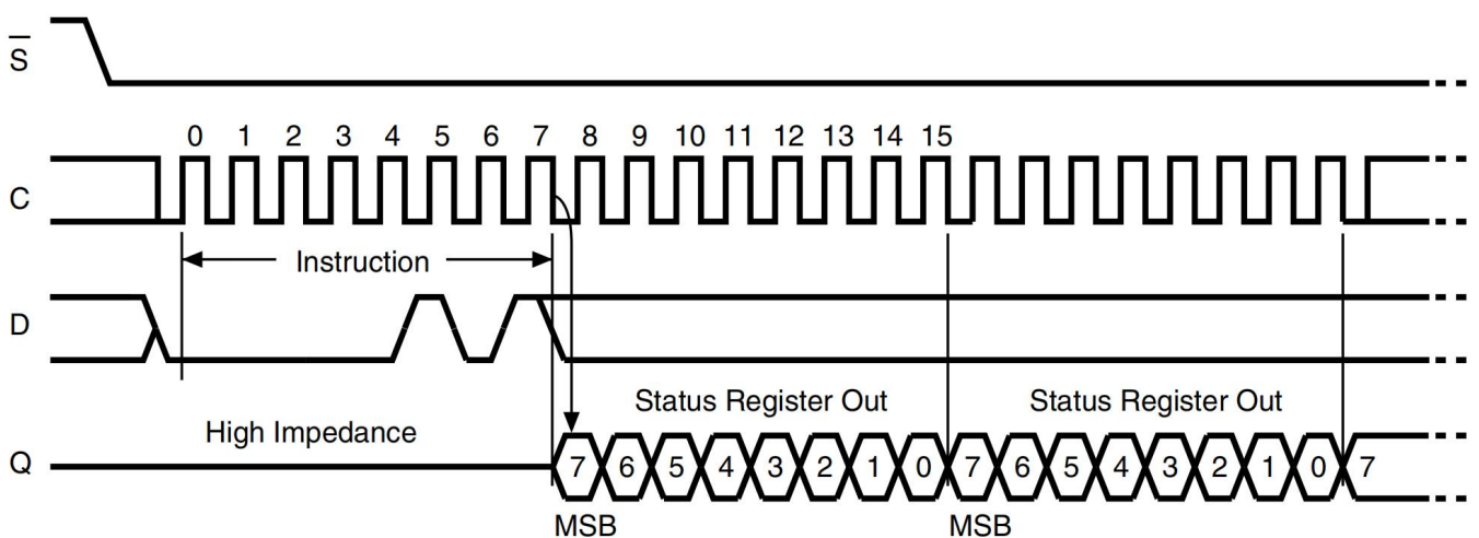
Figure 8. Read Status Register (RDSR) sequence
