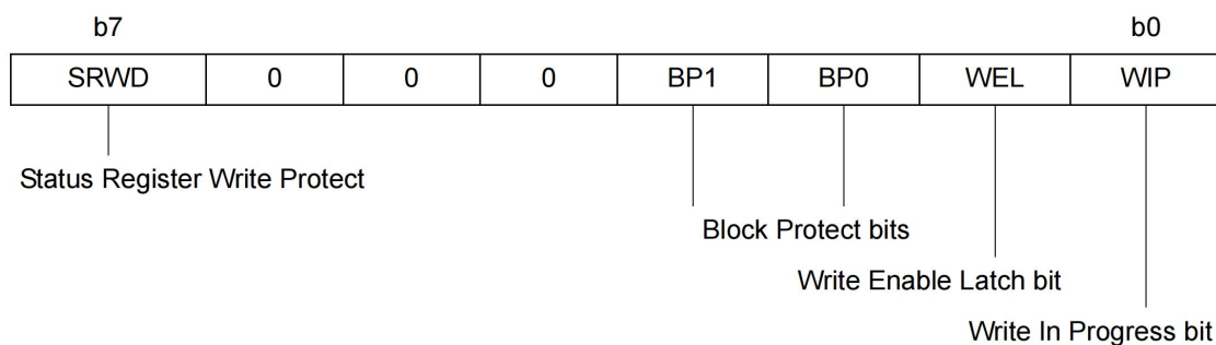
Figure9 . Status Register format
