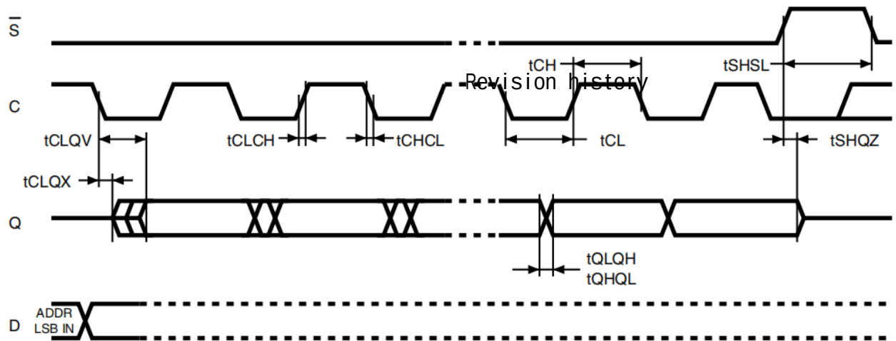
Figure 21. Serial output timing
