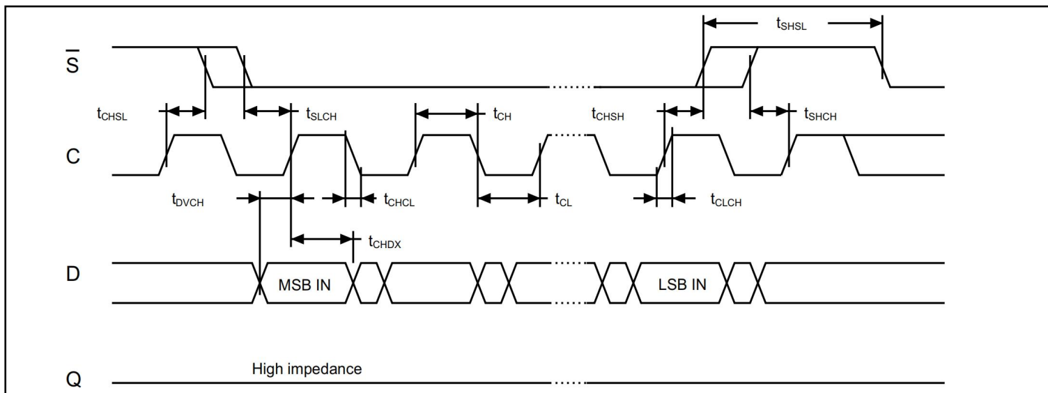
Figure 19. Serial input timing
