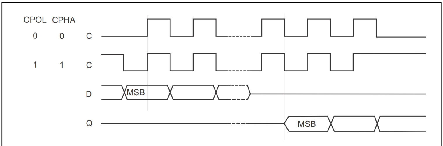
Figure 4. SPI modes supported
