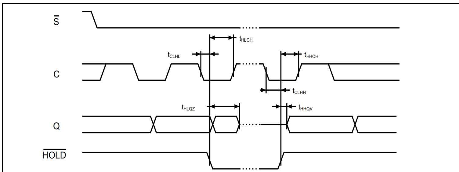
Figure 20. Hold timing
