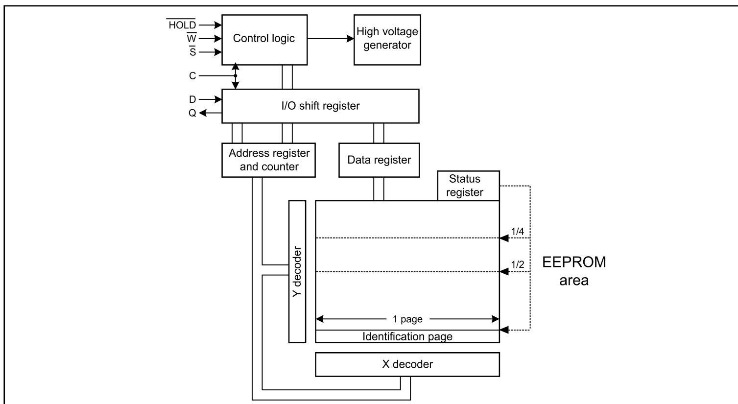
Figure 2. Block diagram
