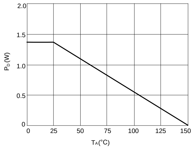
Figure 8: Power De-rating
