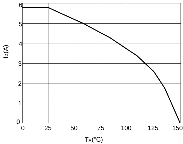
Figure 9: Current De-rating
