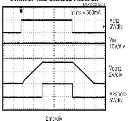
STARTUP AND DISABLE FROM EN
