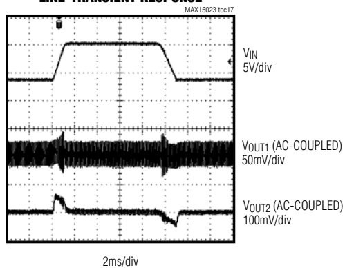
LINE-TRANSIENT RESPONSE
