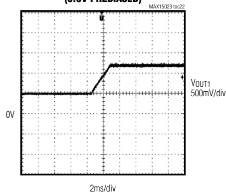
STARTUP INTO PREBIASED OUTPUT (0.5V PREBIASED)
