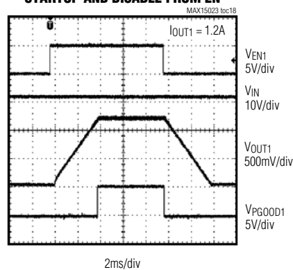
STARTUP AND DISABLE FROM EN
