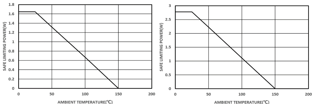
Figure 6. Thermal Derating Curve, Dependence of Safety Limiting Values with Ambient Temperature per VDE (left: \pi 14xU3x ; right: \pi 14xU6x )
