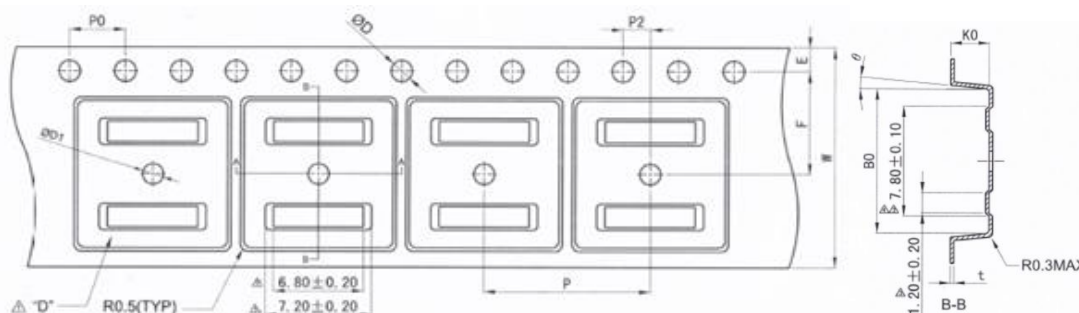
Figure 25.16-Lead Narrow Body SOIC [NB SOIC-16] Reel Information— dimension unit(mm)
