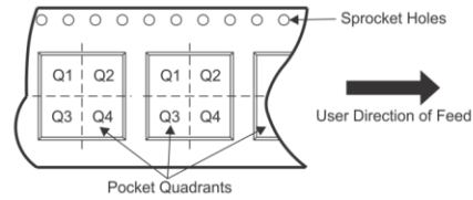
Figure 26.16-Lead Wide Body SOIC [WB SOIC-16] Reel Information
