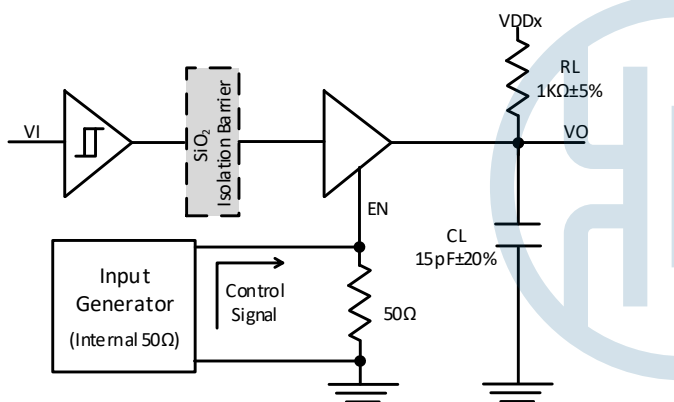
Figure 12. t_{PZL}/t_{PLZ} test circuit
