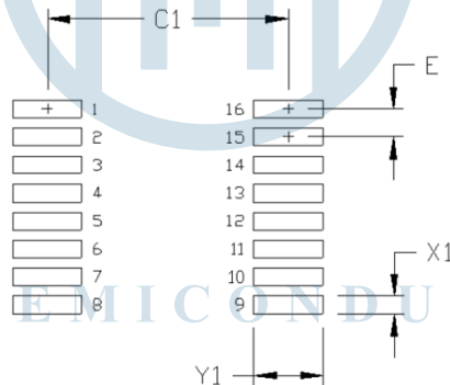
Figure 23. 16-Lead SSOP Land Pattern
