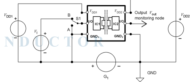
Figure 17. Common-mode transient immunity (CMTI) measurement
