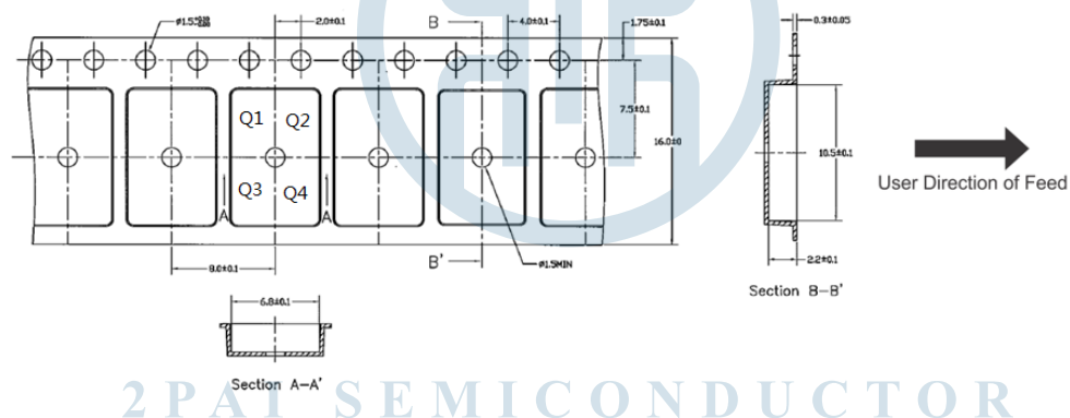
Figure 25.16-Lead Narrow Body SOIC [NB SOIC-16] Reel Information— dimension unit(mm)
