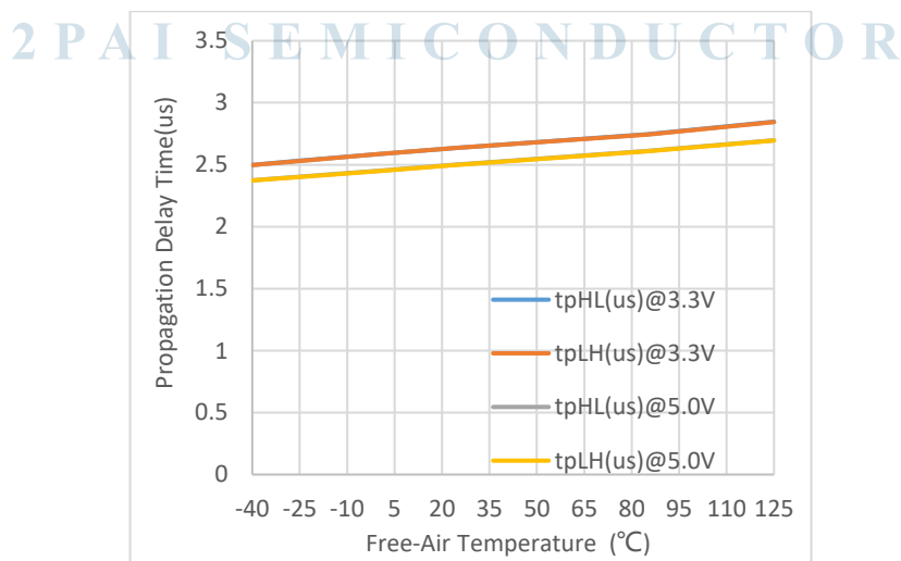
Figure 9. \pi 14xU6x Propagation Delay Time vs. Free-Air Temperature
