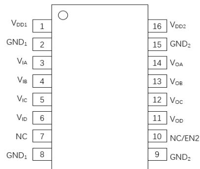
Figure 3. \pi 140Uxx Pin Configuration
