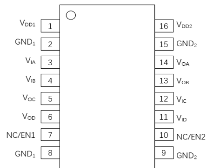
Figure 5. \pi 142Uxx Pin Configuration
