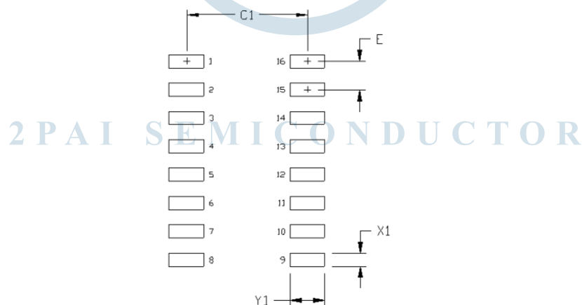
Figure 21.16-Lead Narrow Body SOIC [NB SOIC-16] Land Pattern
