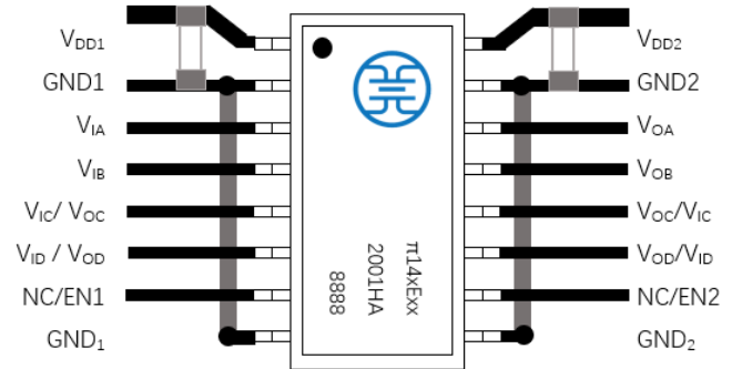
Figure 16. Recommended Printed Circuit Board Layout
