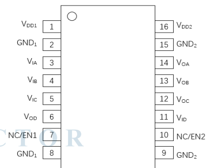
Figure 4. \pi 141Uxx Pin Configuration
