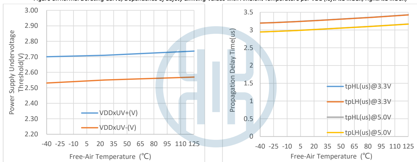
Figure 7. UVLO vs. Free-Air Temperature
