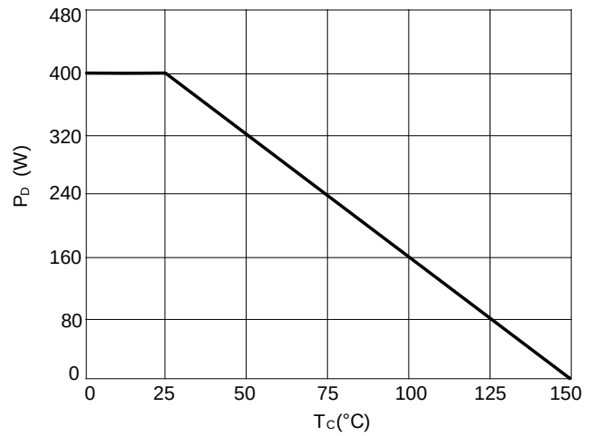
Figure 10: Power De-rating
