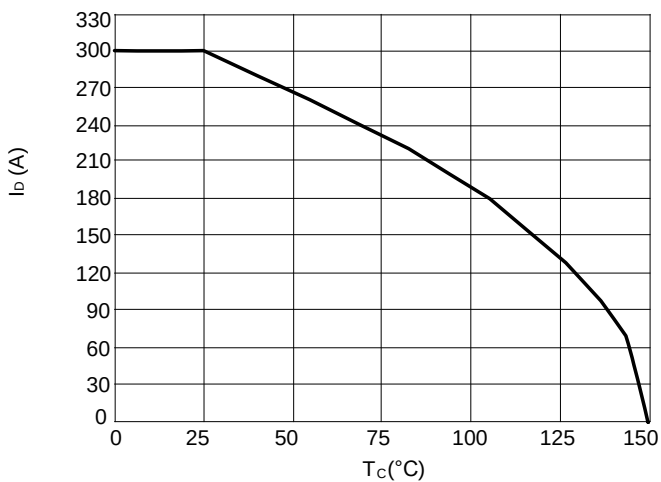
Figure 11: Current De-rating
