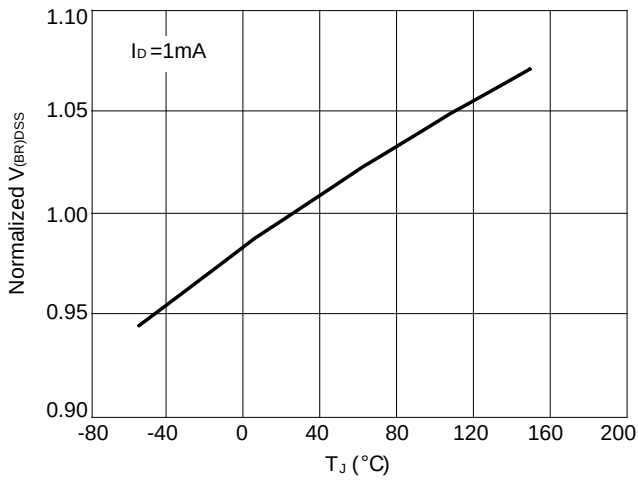
Figure 7: Normalized Breakdown Voltage vs Junction
