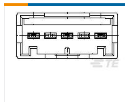
TE Part #2013485-1 GIC 2.5 HDR ASSY TIN VERSION 3/5P
