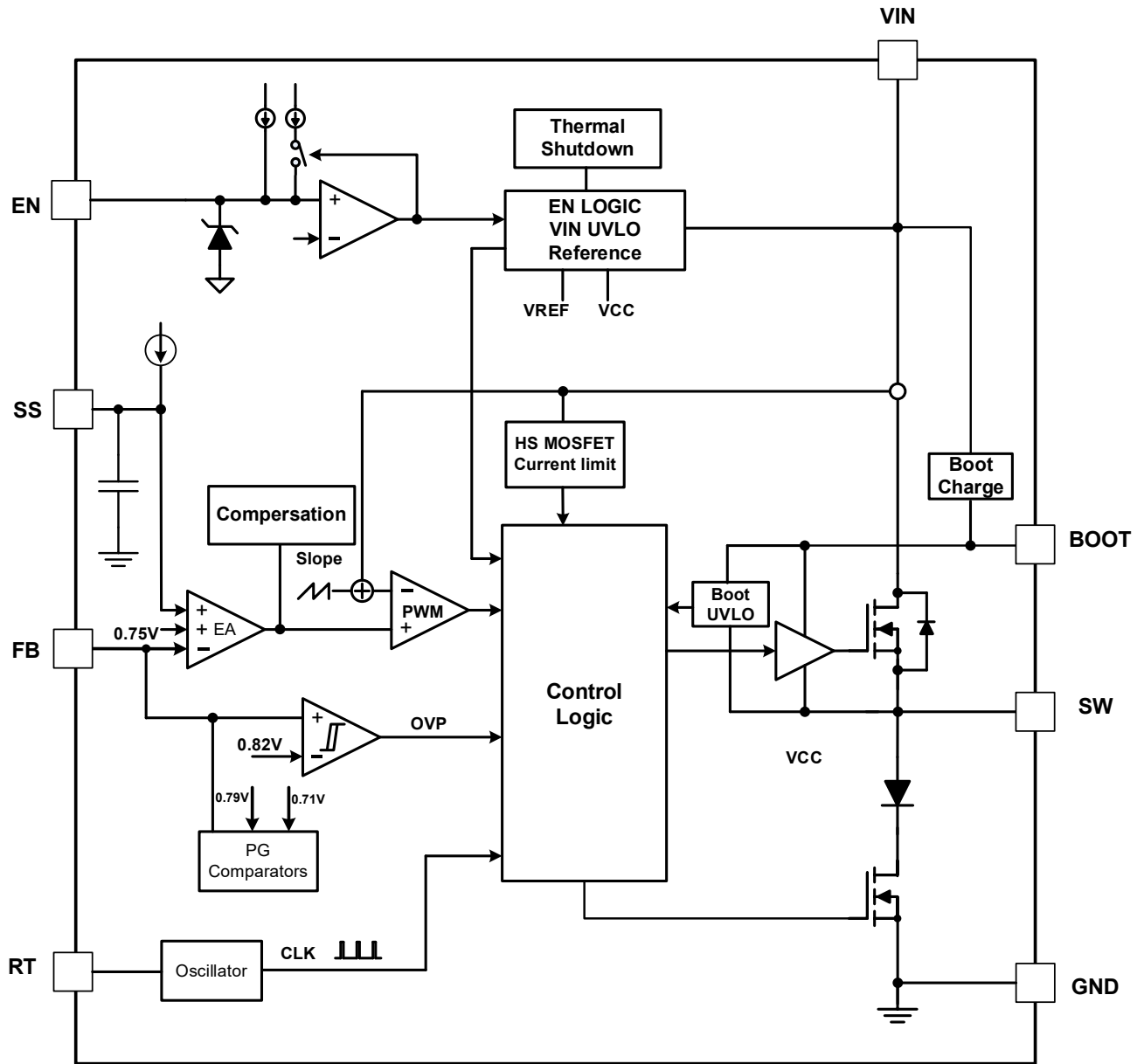
Figure 5 Block Diagram of TPS54360BDDAR
