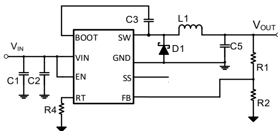
Simplified Schematic
