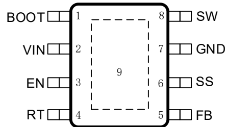
Top View: TPS54360BD eSOP-8L
