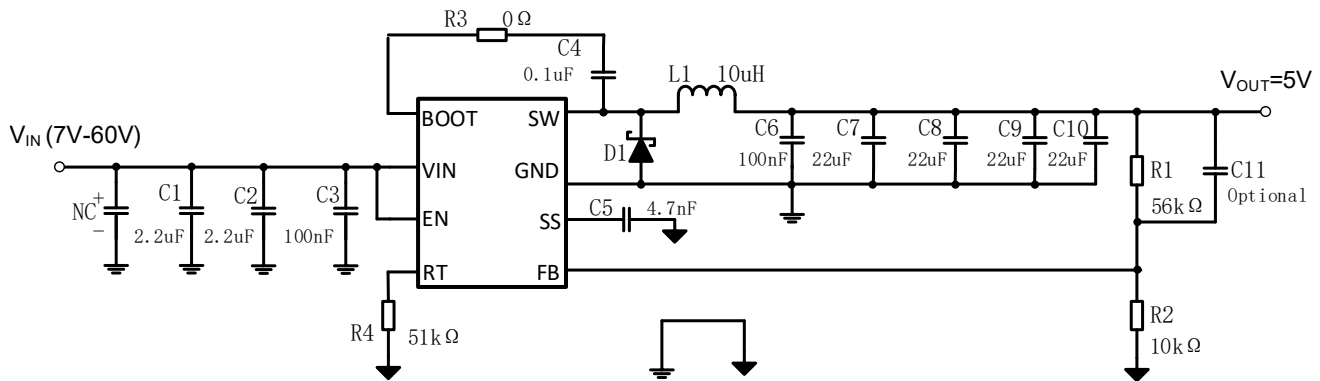
Figure 7. 24V INPUT, 5V/3A OUTPUT
