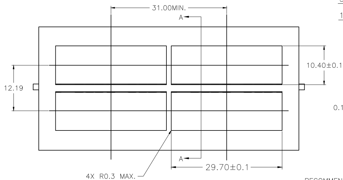
RECOMMENDED BEZEL DESIGN BELLY TO BELLY APPLICATIONS
