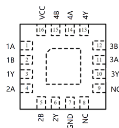
QFN-16 3*3
