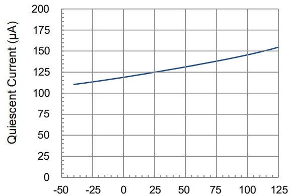
Quiescent Current as a function of Temperature.
