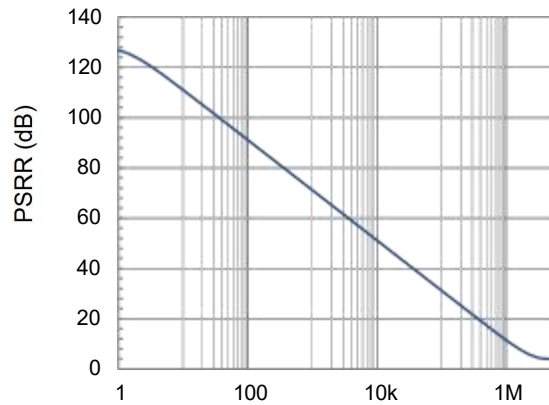
Power Supply Rejection Ratio as a function of Frequency.
