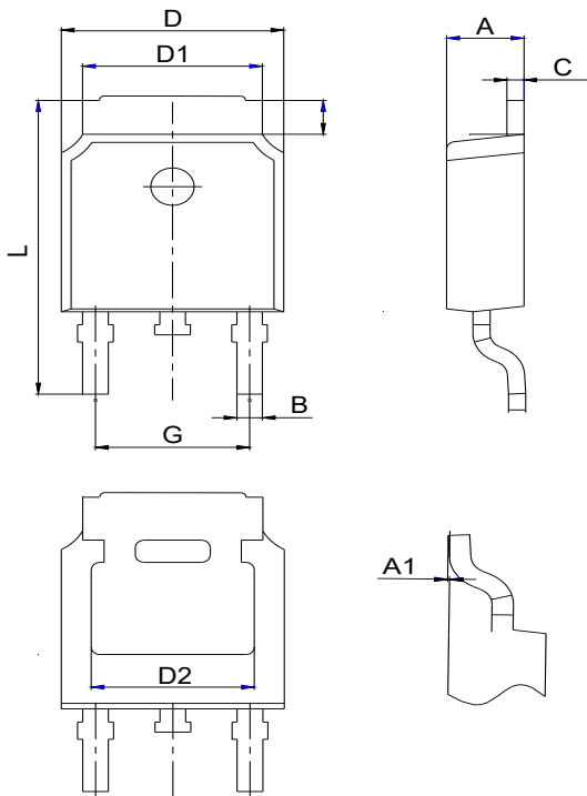
TO-252
