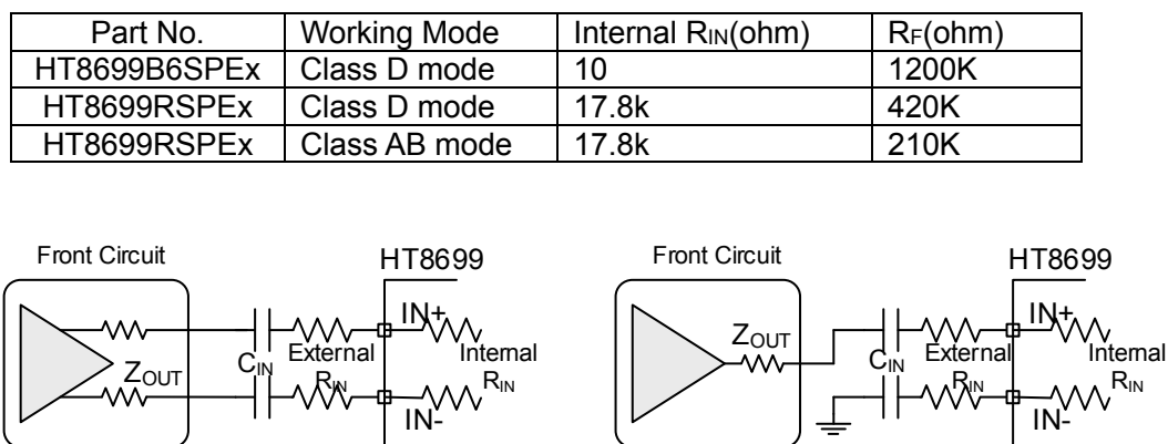
Fig. 3 (1) Differential Input;
